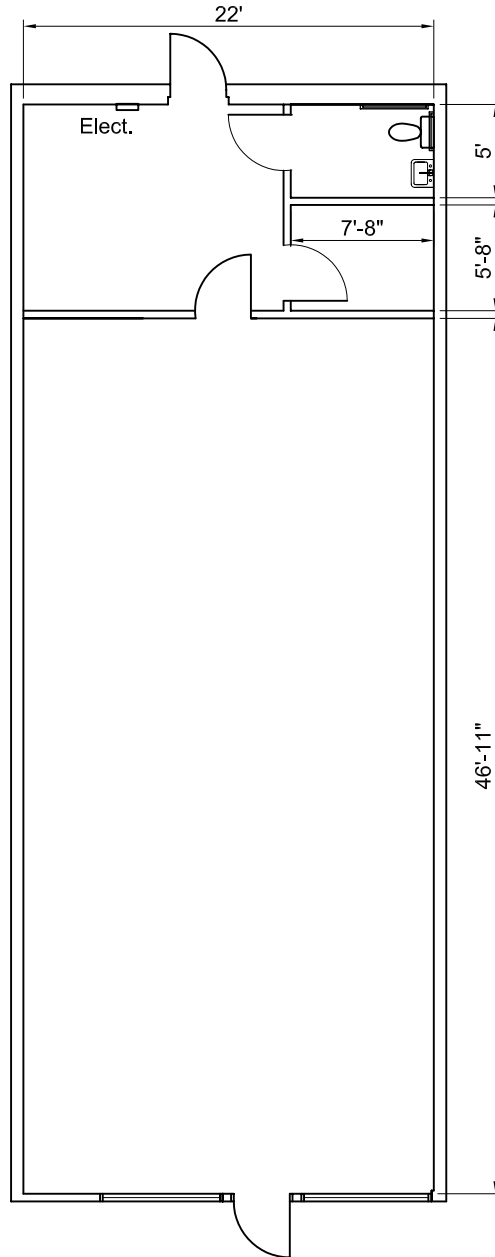
Floor Plan Suite 7 No Scale 1,363 SF
